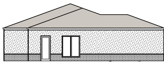
Typical East/West Elevation
