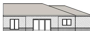
Typical South Elevation
